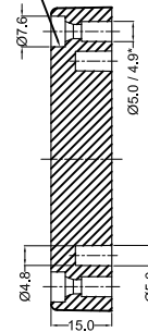
SECTION C-C
