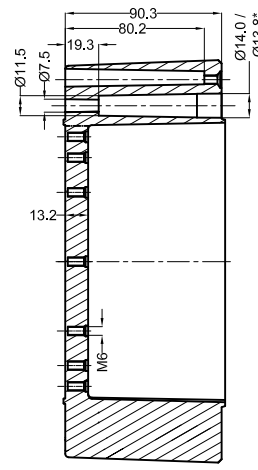
SECTION B-B
